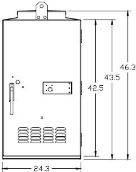
5.3 – Model 356i ATC Cabinet Housing Rear View
