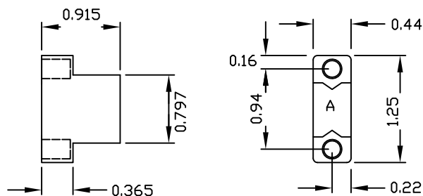
CONNECTOR C2S
