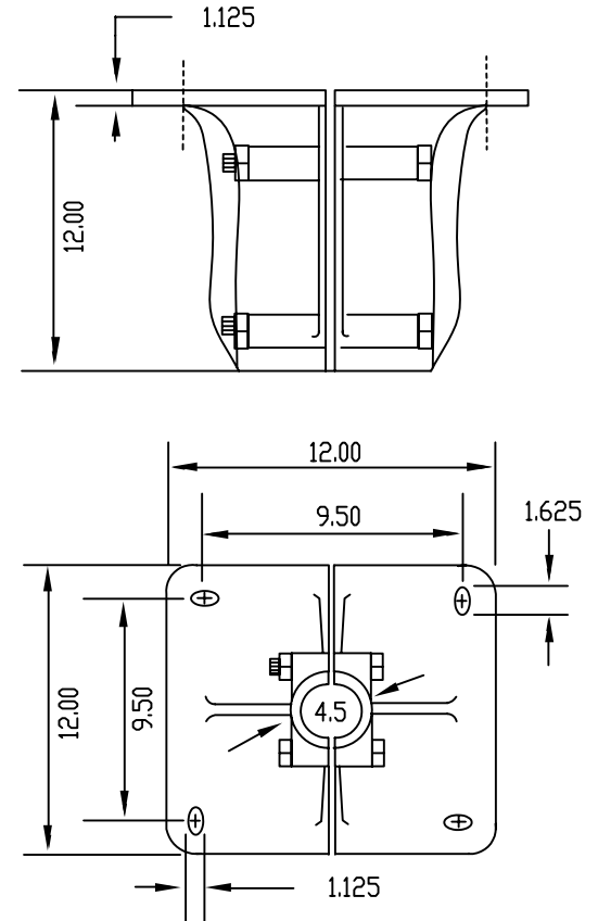
SLIPFITTER (CAST ALUMINUM) DETAIL
