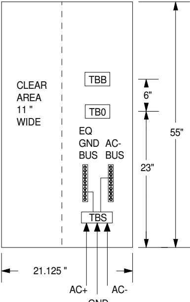
332 SERVICE PANEL No. 1
