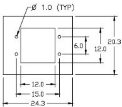
5.1 – Model 356i ATC Cabinet Housing Base
