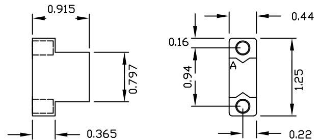
CONNECTOR C2S
