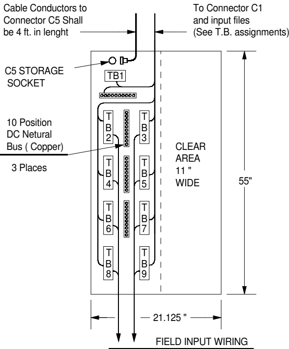
332 INPUT PANEL No. 1
