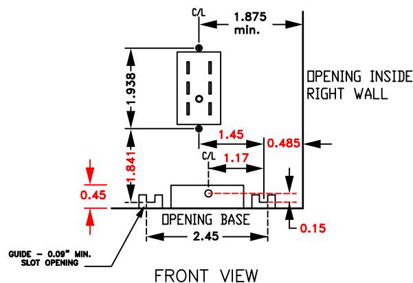
POWER SUPPLY CONNECTOR/STUD MOUNTING DETAIL
