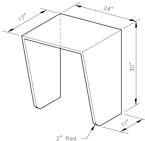
VISOR ENCLOSURE
