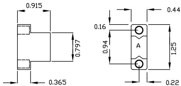
CONNECTOR C2S
