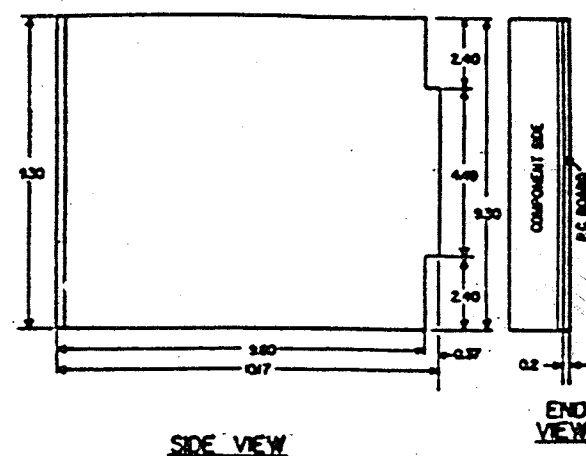
MODEL 210 MONITOR UNIT
