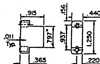
CONNECTOR C2S
