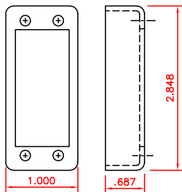
HOOD FOR C1P
