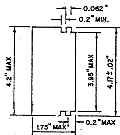
MODEL 200 & 204 CROSS SECTION
