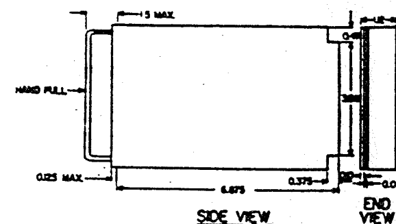
DETAIL FOR MODELS 222, 224, 227 228, 231, 232, 234, 242, 244, 252 & 255
