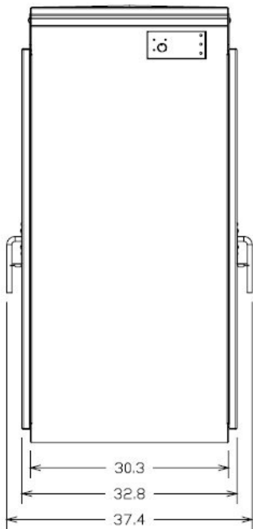
5.2 - 352i ATC Cabinet Housing Side View
