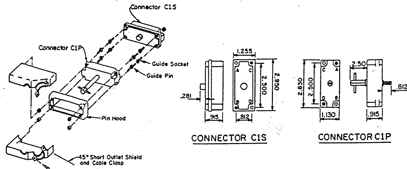
CONNECTOR C1 DETAIL
