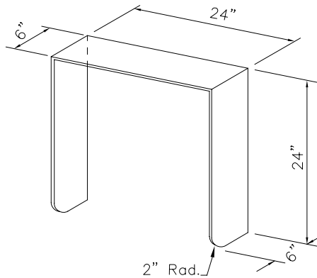
(Pedestrian Head Sign)
