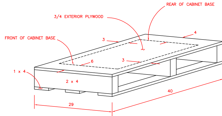
CABINET PALLET
