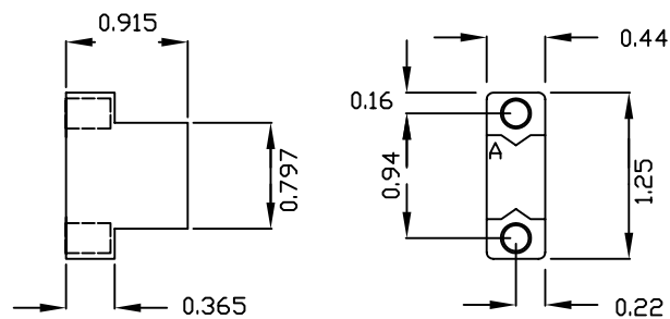
CONNECTOR C2S
